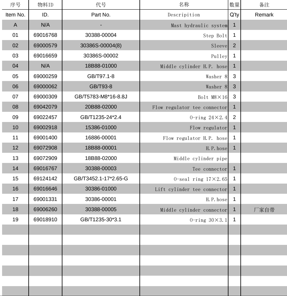
门架管路系统(三级全自由二联) MAST HYDRAULIC SYSTEM(FULL FREE 3-STAGE MAST Two-THROW)
