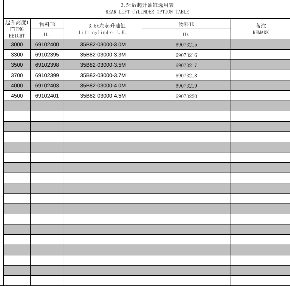
后起升油缸(二级全自由)/REAR LIFT CYLINDER(FULL FREE 2-STAGE MAST)
