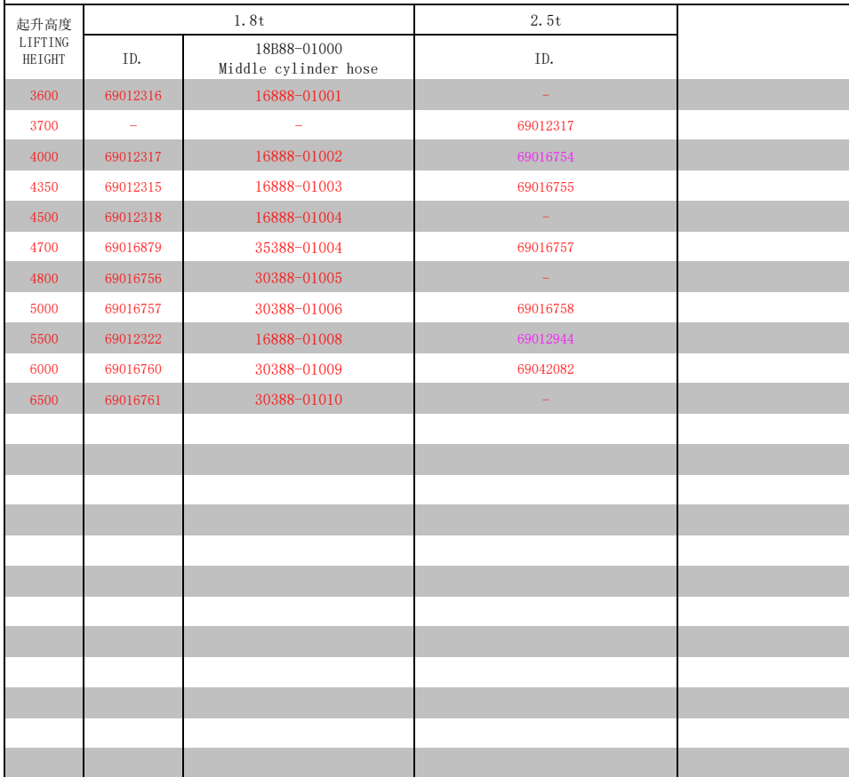
门架管路系统(三级全自由二联) MAST HYDRAULIC SYSTEM(FULL FREE 3-STAGE MAST Two-THROW)
