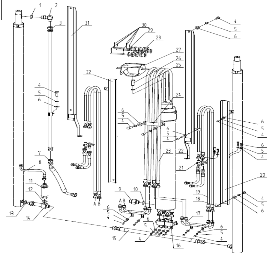
门架管路系统(二级全自由四联) MAST HYDRAULIC SYSTEM(FULL FREE 2-STAGE MAST FOUR THROW)
