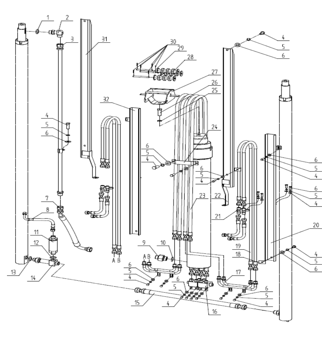
图72/Fig72. 门架管路系统(二级全自由四联) MAST HYDRAULIC SYSTEM(FULL FREE 2-STAGE MAST FOUR THROW)
