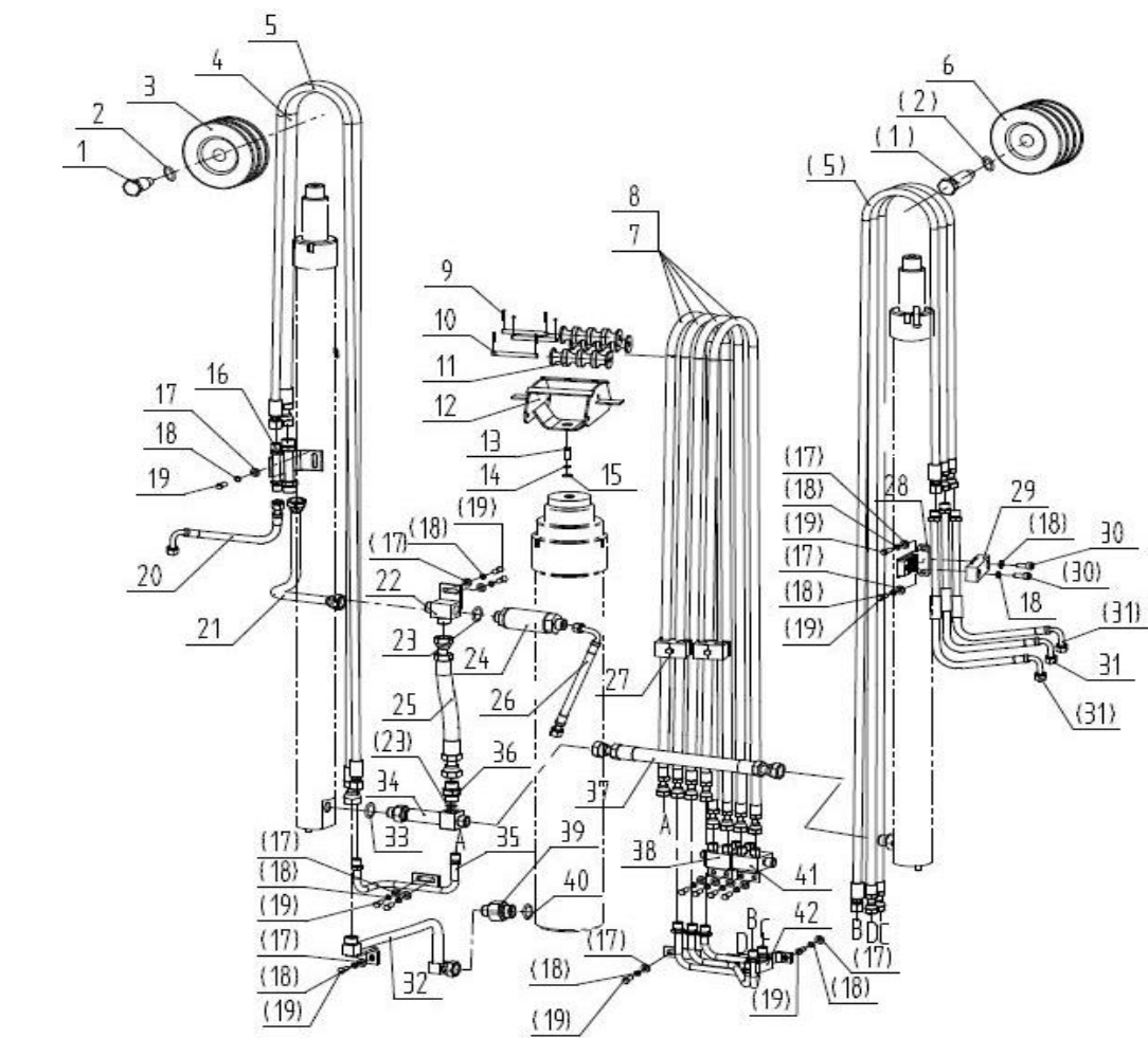
图75/Fig75. 门架管路系统(三级全自由四联) MAST HYDRAULIC SYSTEM(FULL FREE 3-STAGE MAST FOUR THROW)
