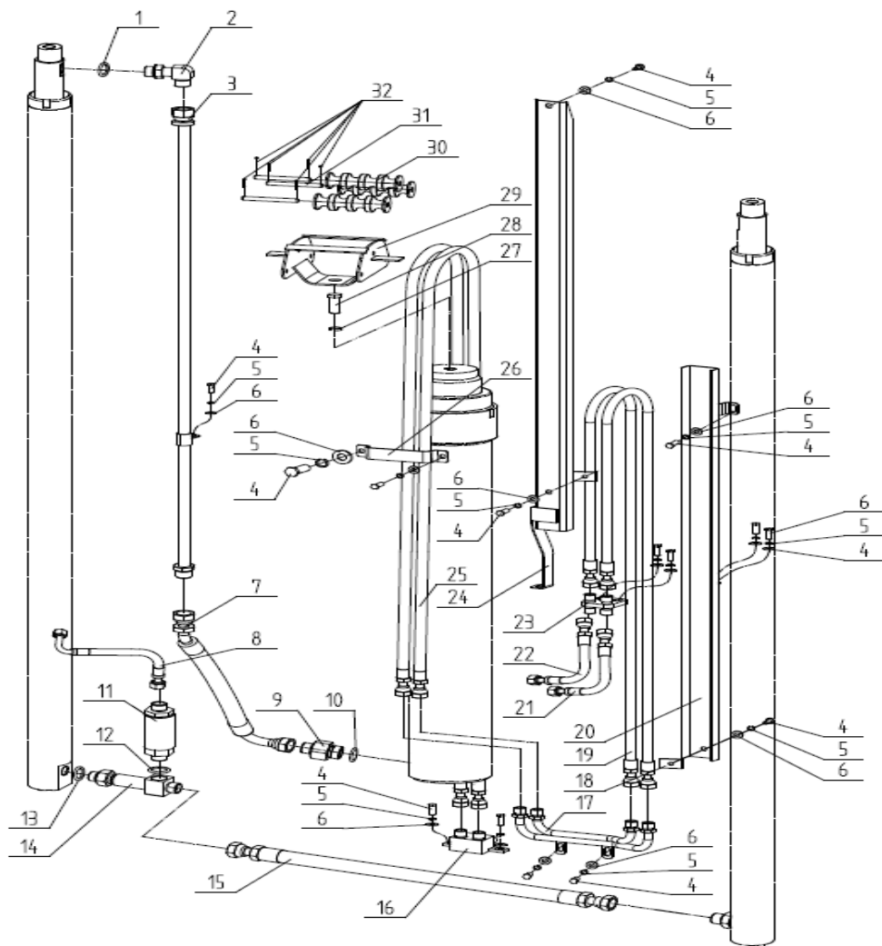
门架管路系统(二级全自由三联) MAST HYDRAULIC SYSTEM(FULL FREE 2-STAGE MAST THREE THROW)
