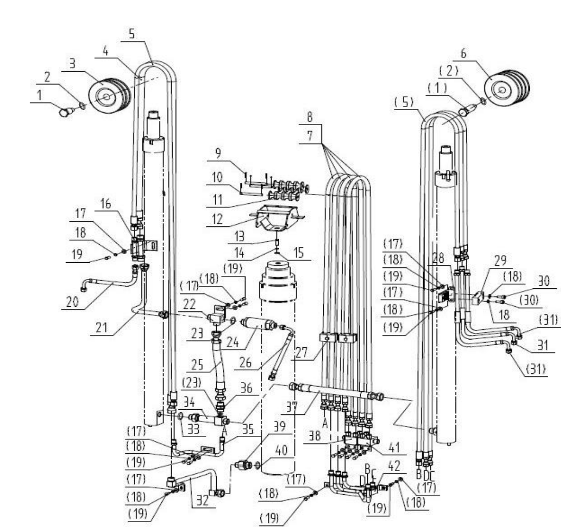
图75/Fig75. 门架管路系统(三级全自由四联) MAST HYDRAULIC SYSTEM(FULL FREE 3-STAGE MAST FOUR THROW)
