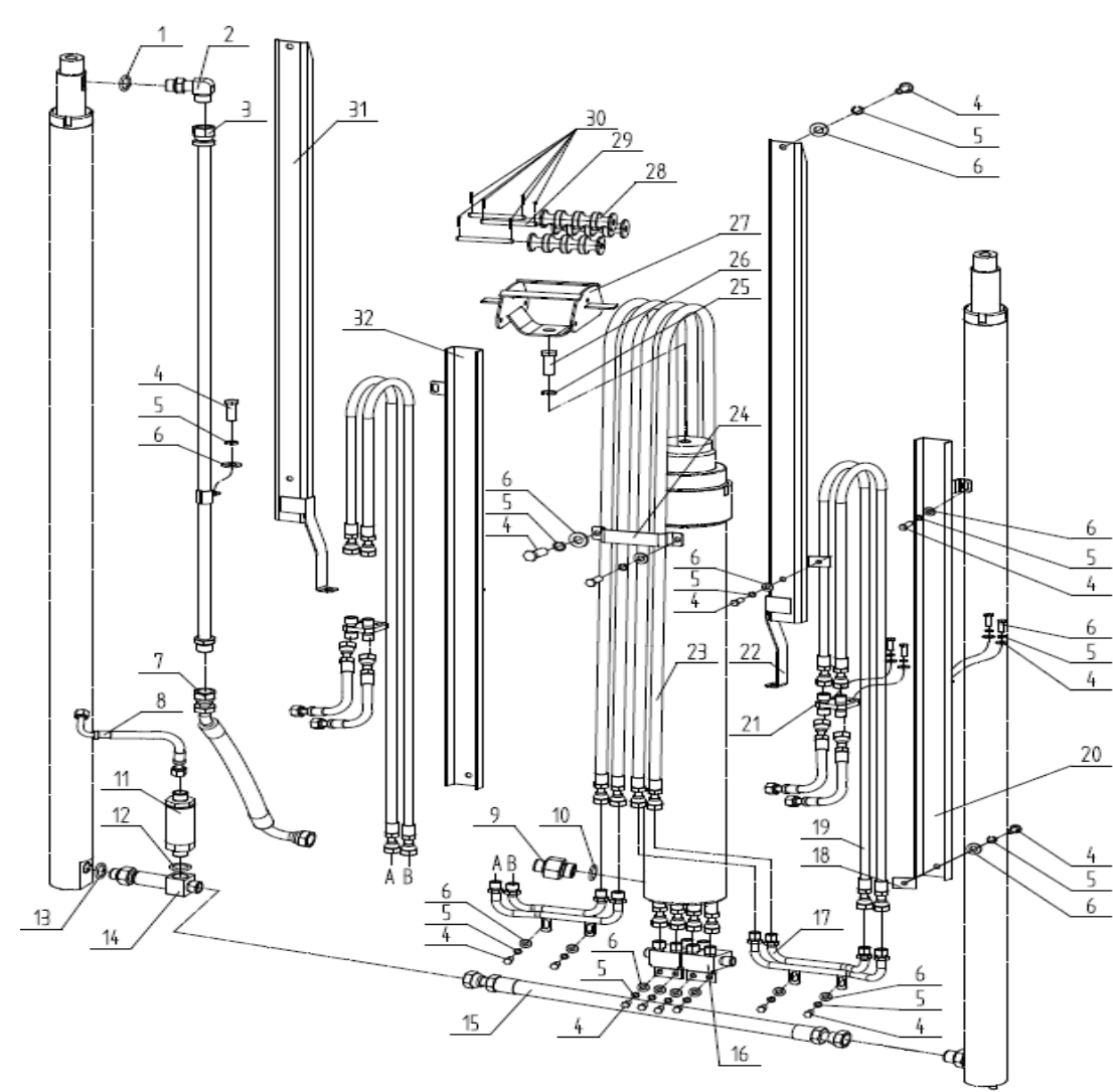
图72/Fig72. 门架管路系统(二级全自由四联) MAST HYDRAULIC SYSTEM(FULL FREE 2-STAGE MAST FOUR THROW)
