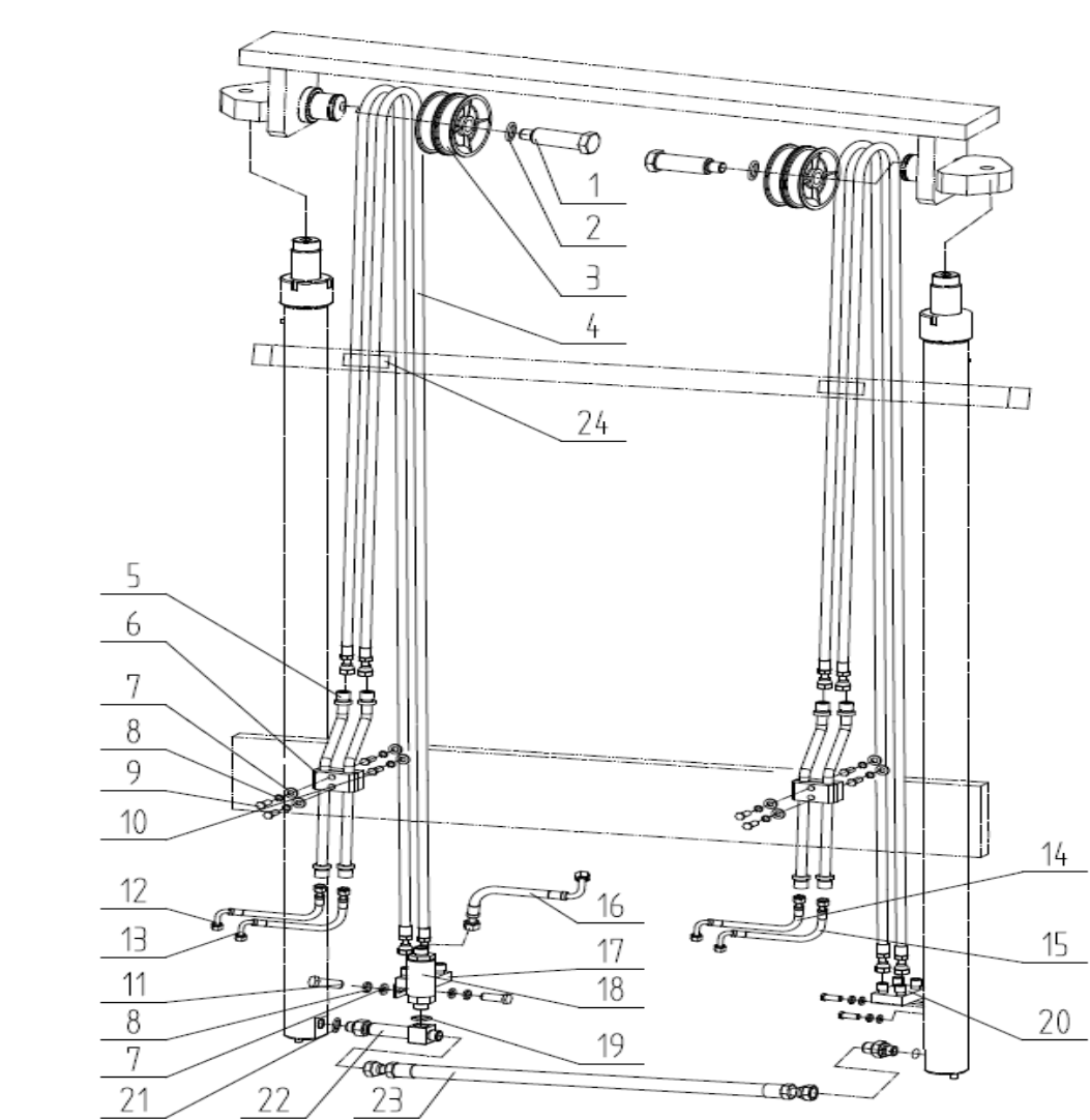
图69/Fig69. 门架管路系统(基本型四联)/MAST HYDRAULIC SYSTEM(NORMAL MAST FOUR THROW)
