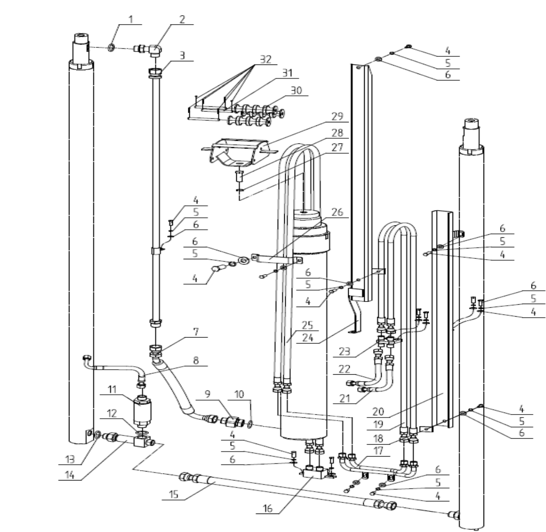
图71/Fig71. 门架管路系统(二级全自由三联) MAST HYDRAULIC SYSTEM(FULL FREE 2-STAGE MAST THREE THROW)
