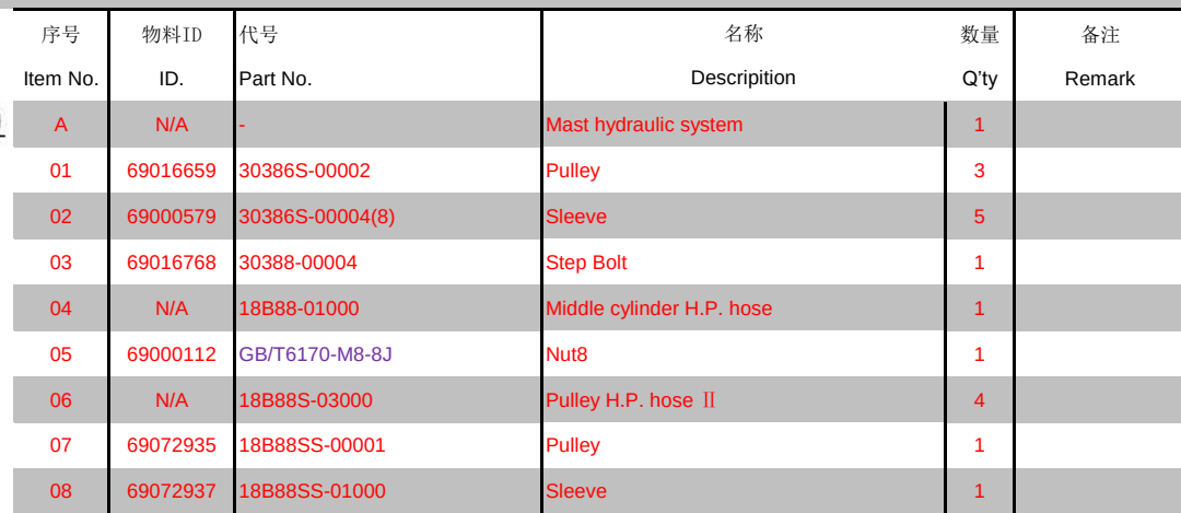
门架管路系统(三级全自由四联) MAST HYDRAULIC SYSTEM(FULL FREE 3-STAGE MAST Four-THROW)
