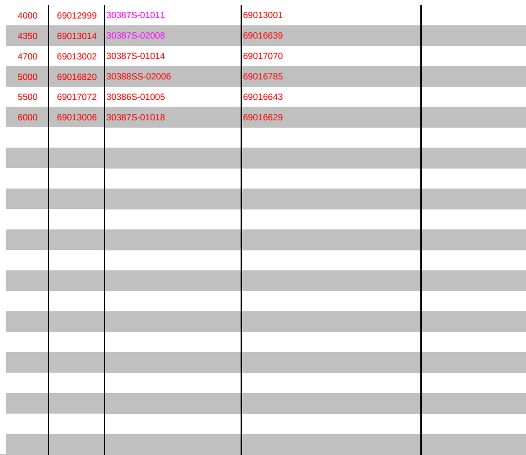
门架管路系统(三级全自由四联) MAST HYDRAULIC SYSTEM(FULL FREE 3-STAGE MAST Four-THROW)
