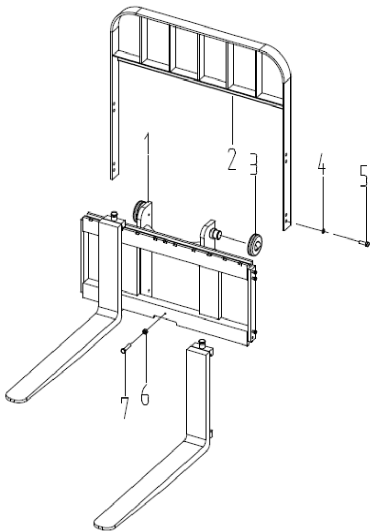
图41/FIG. 41 货叉架(二级全自由)/LIFT BRACKET (FULL FREE 2 STAGE MAST)
