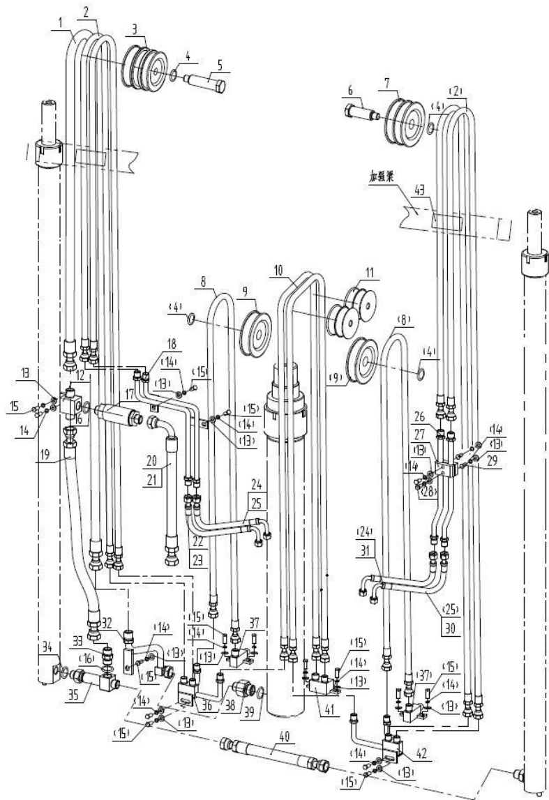
图79/Fig. 79 门架管路系统(三级全自由四联)/MAST HYDRAULIC SYSTEM(FULL FREE 3-STAGE MAST FOUR-THROW)
