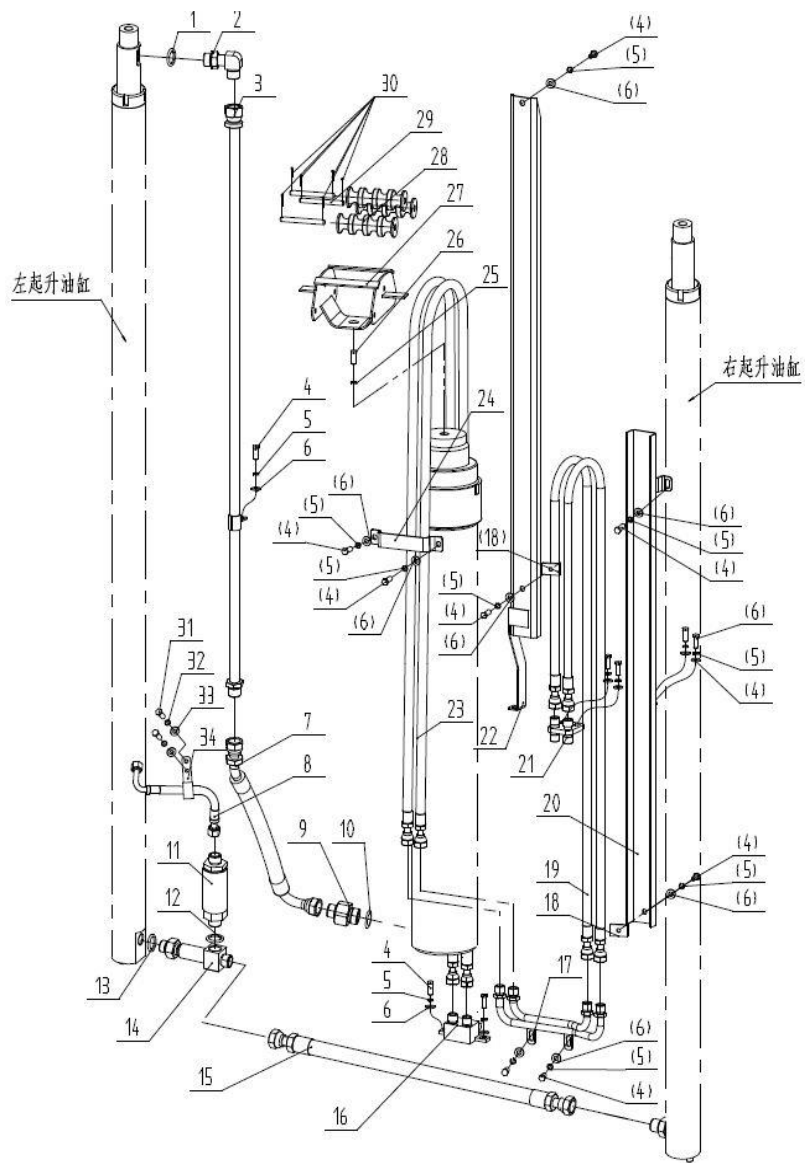
门架管路系统(两级全自由四联)/MAST HYDRAULIC SYSTEM(FULL FREE 2-STAGE MAST FOUR-THROW)
