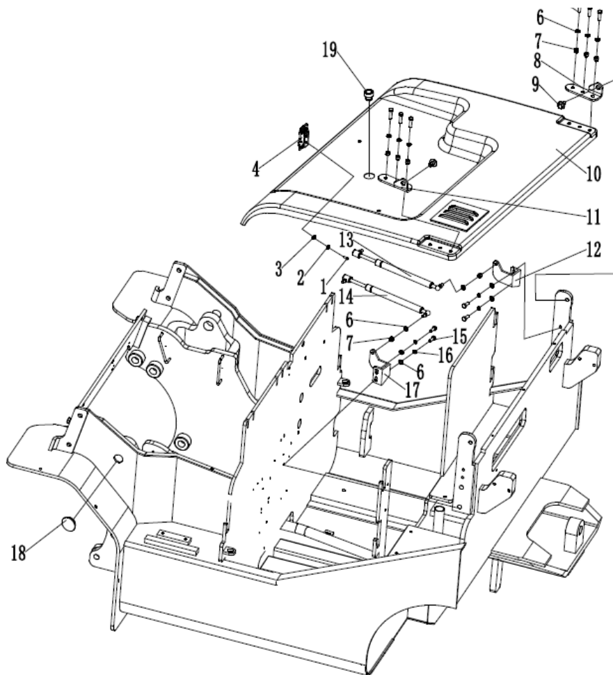
图28/Fig. 28 仪表架及机罩安装/ DISPLAY BRACKET AND HOOD INSTALLATION
