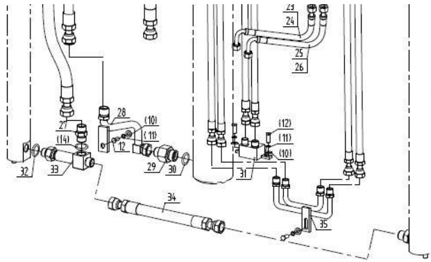
门架管路系统(三级全自由三联)/MAST HYDRAULIC SYSTEM(FULL FREE 3-STAGE MAST THREE-THROW)
