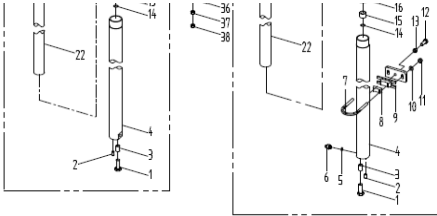
起升油缸(基本型)/LIFT CYLINDER(NORMAL MAST)
