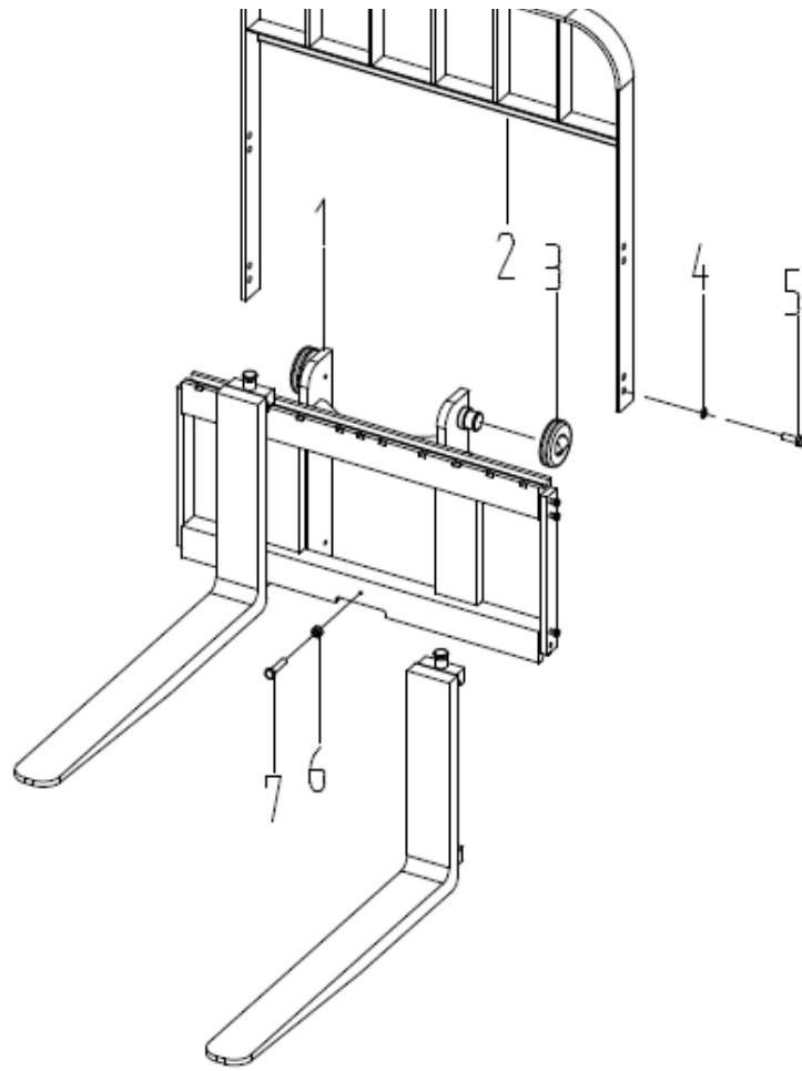
图42/FIG. 42 货叉架(三级全自由)/LIFT BRACKET (FULL FREE 3 STAGE MAST)
