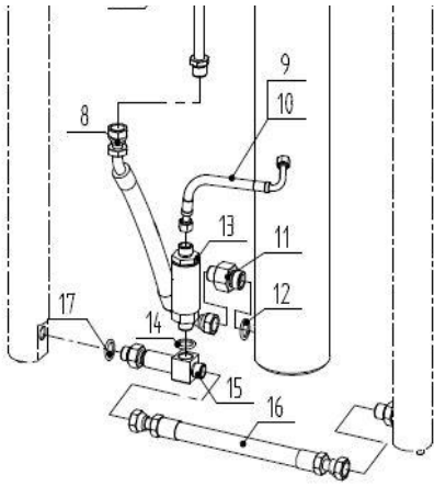
图69/ Fig. 69 门架管路系统(两级全自由二联)/MAST HYDRAULIC SYSTEM(FULL FREE 2-STAGE MAST TWO-THROW)
