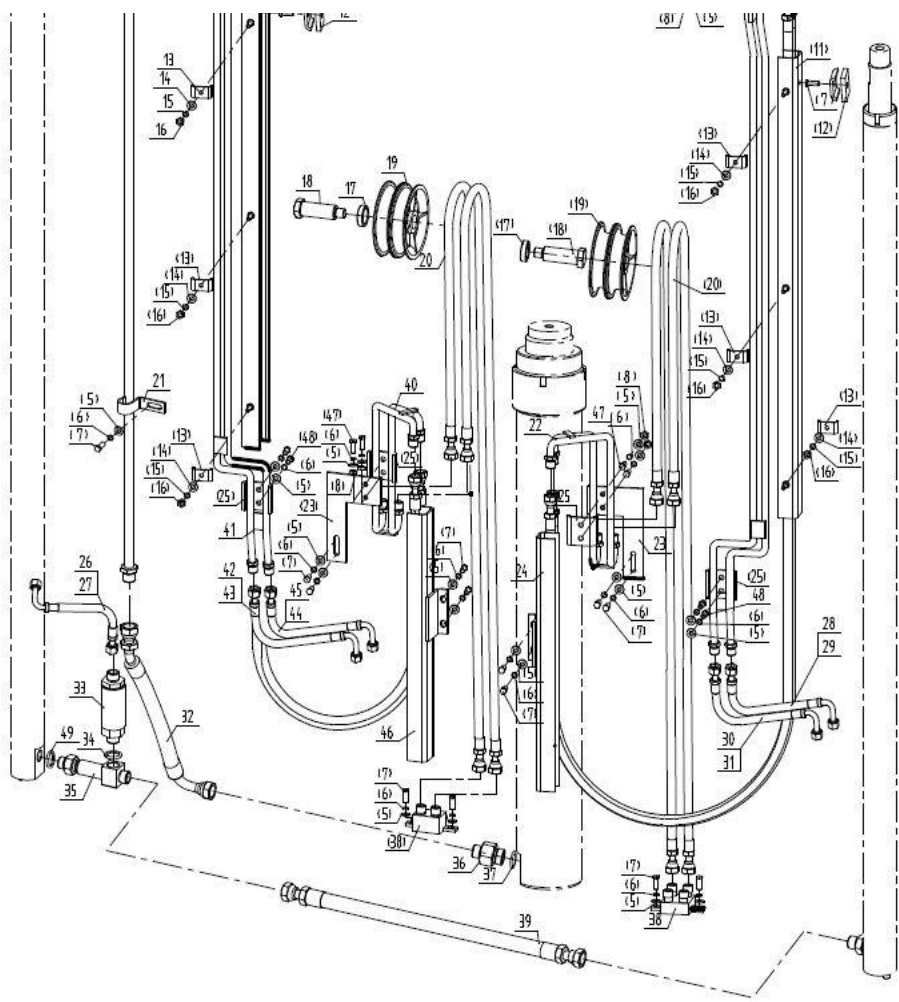
图72/Fig. 72 门架管路系统(两级全自由四联)/MAST HYDRAULIC SYSTEM(FULL FREE 2-STAGE MAST FOUR-THROW)
