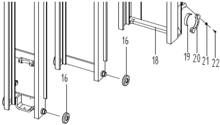
起升油缸(基本型)/LIFT CYLINDER(NORMAL MAST)
