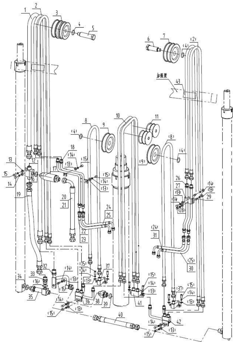
图78/Fig. 78 门架管路系统(三级全自由四联)/MAST HYDRAULIC SYSTEM(FULL FREE 3-STAGE MAST FOUR-THROW)
